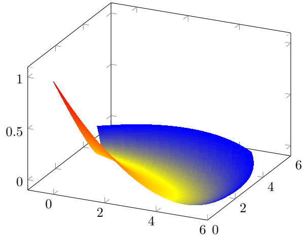
Biquadratic Shape (Shading Type 6, one patch)
